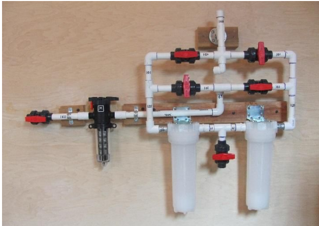
BACKFLUSH LEFT FILTER POSITION
